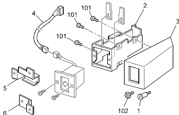
Optional Counter Interface Unit Type A (B870-11)
