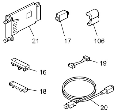
Card Reader Bracket Type1075 (B498-01)
