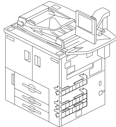
30. Paper Feed Unit 3 (D059/D060/D061)
