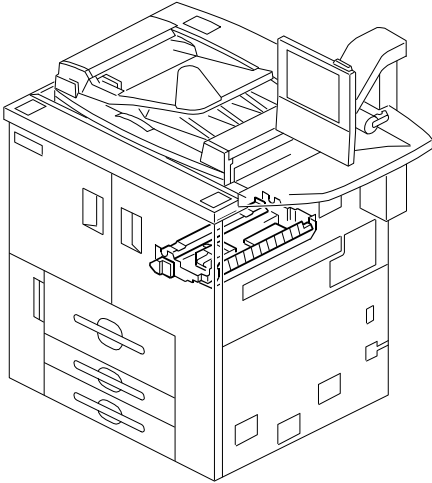
49. Transfer Belt Unit 2 (D059/D060/D061)
