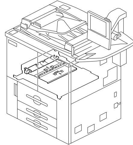
63. Duplex Unit 6 (D059/D060/D061)
