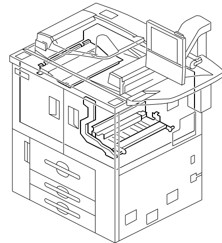
84. Frame Section 3 (D059/D060/D061)
