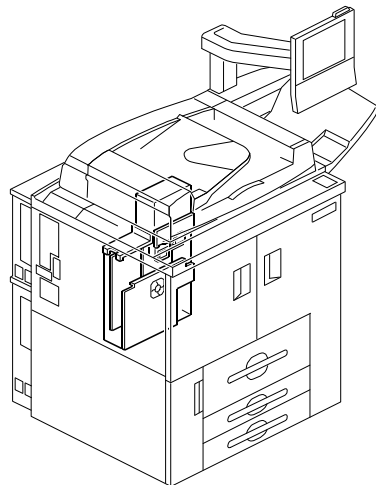
73. Electrical Section 2 (D059/D060/D061)
