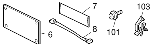
Copy Data Security Unit Type F (B829-07)
