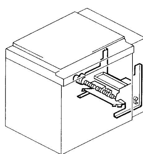
17. PAPER FEED AND REGISTRATION 5 (A105)
