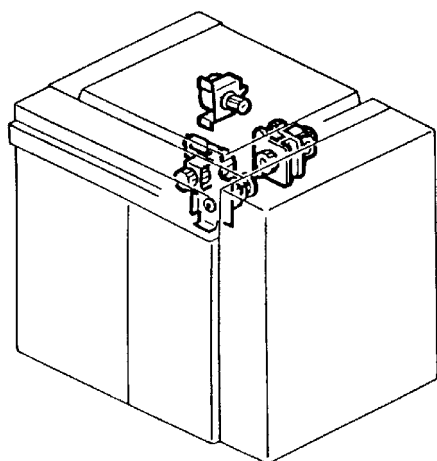
28. TRANSFER/DEVELOPMENT DRIVE SECTION (A105)
