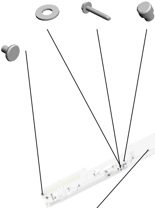
12.AA143802 (x4) SCREW:6X1.7
