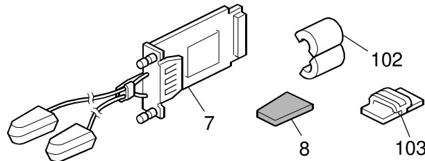
IEEE802.11a/g Interface Unit Type J/K (D377-01/02/19)
