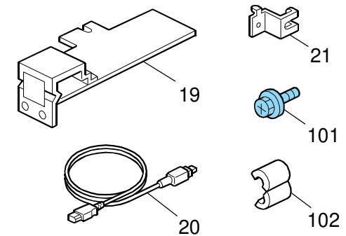
Interface PCB Type W7140 (D445-17)
