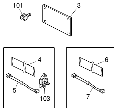
Copy Data Security Unit Type F (B829-07)
