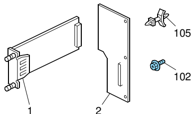
Copy Data Security Unit Type F (B829-07)
