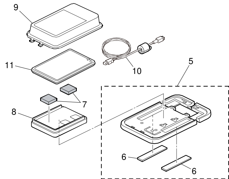
NFC Card Reader Type M19 (D3BS-21)
