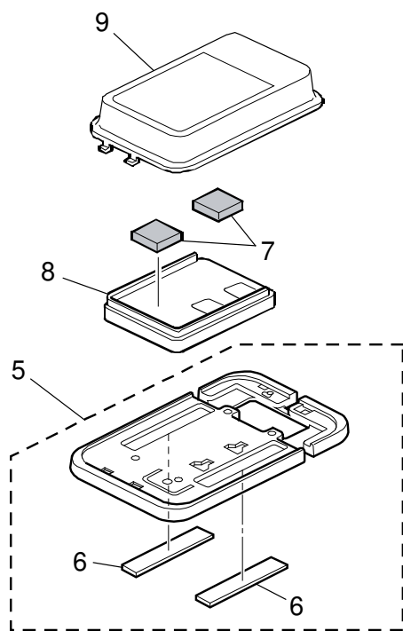
Smart Card Reader Built-in Unit Type S6 (D3DH-07)
