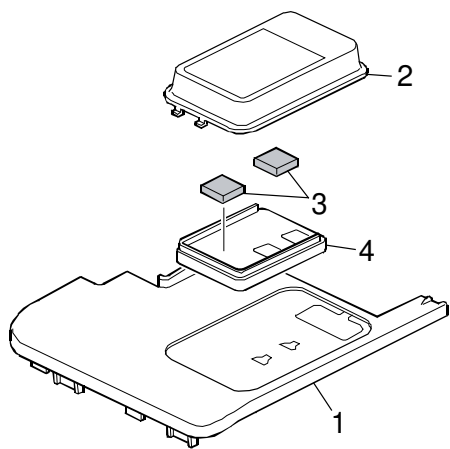
Smart Card Reader Built-in Unit Type M19 (D3BS-22)
