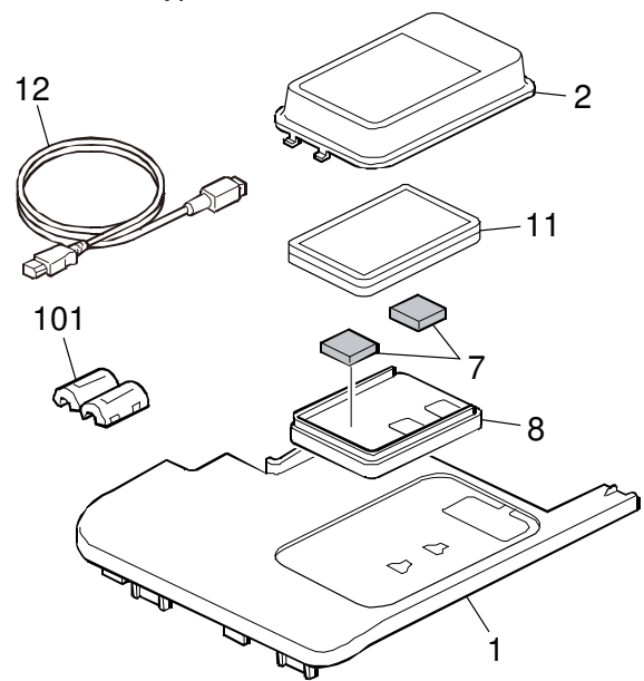
NFC Card Reader Type M19 (D3BS-21)
