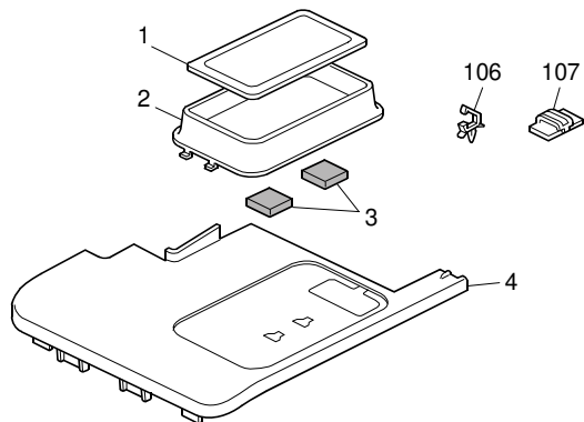
Key Counter Bracket Type1027 (B452-57)
