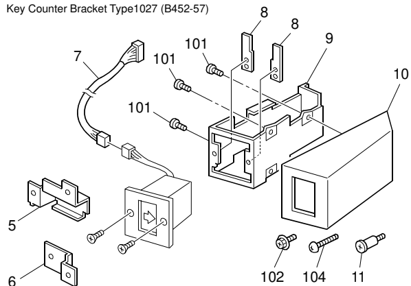
Key Counter Bracket Type1027 (B452-57)
