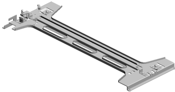
92.D0141751 CARRIAGE:NO.1
