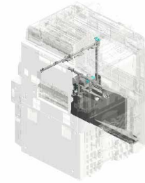
U016 TONER COLLECTION
