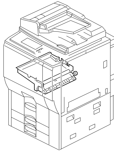
41. Transfer Belt Cleaning 1 (D014/D015)
