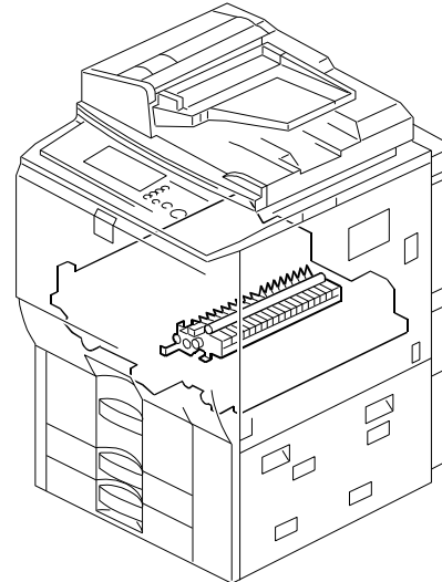
47. Paper Transfer 1 (D014/D015)
