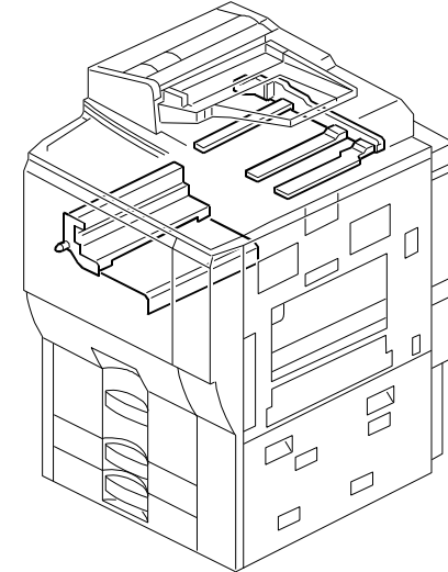
81. Frame Section 1 (D014/D015)
