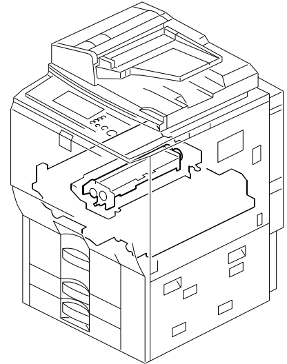
54. Fusing Unit 6 (D014/D015)
