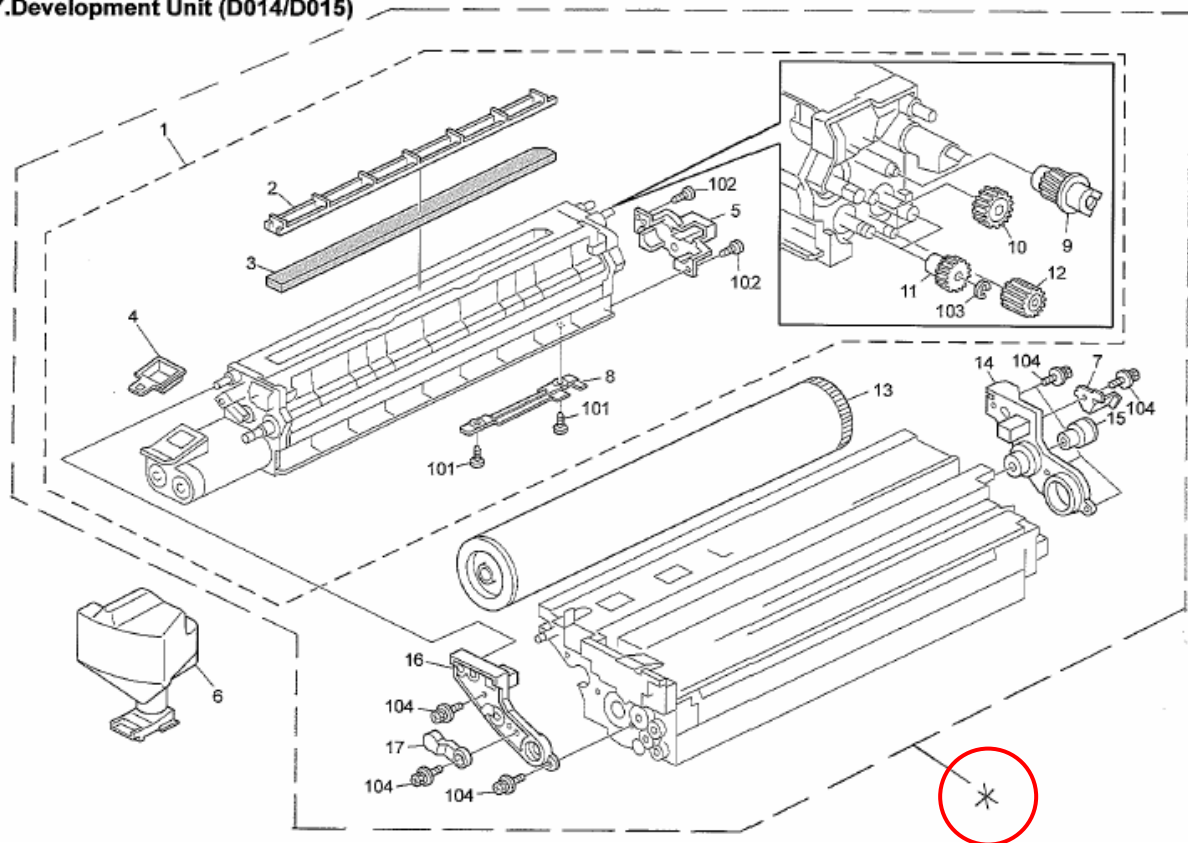
37.Development Unit (D014/D015)
