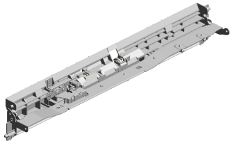
207.D1504742 (C6003):GUIDE PL ATE:VERTICAL TR ANSPORT:DRIVEN: PAPER THICK:ASS' Y 201507-20 O/O
