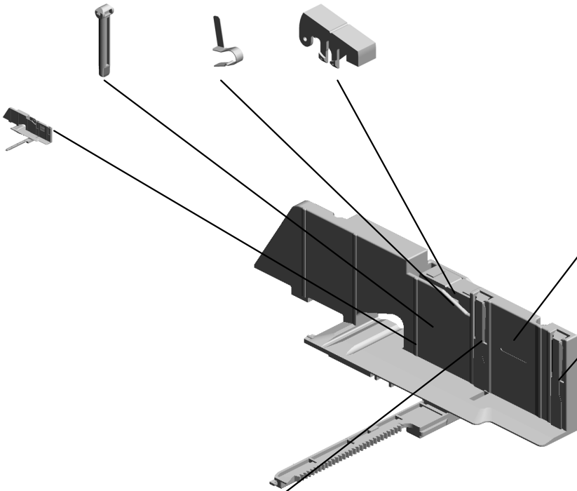
28.B2232932 SIDE FENCE:REAR :UNIVERSAL:NO.2
