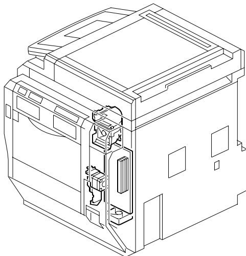
46. Drive Section 3 (B222/B224)
