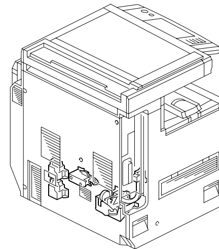
45. Drive Section 2 (B222/B224)
