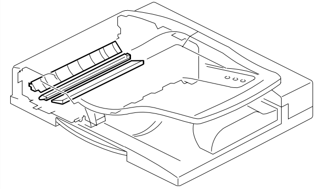
9. Original Transfer 1 (B222/B224)
