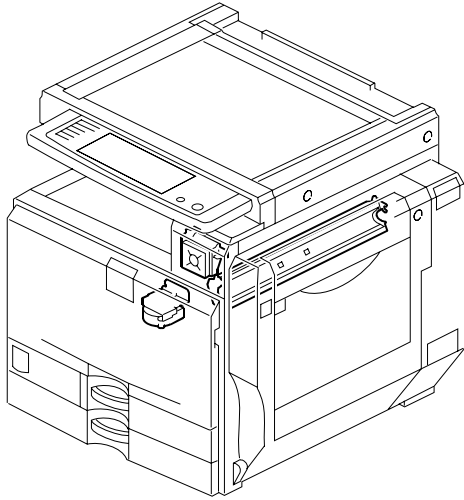
31. Fusing unit 3 (B222/B224)
