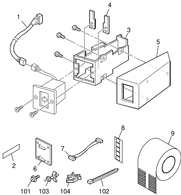
Optional Counter Interface Unit Type A
