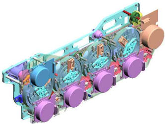
57.D0251100 DRIVE UNIT:ENGINE:ATHENA-C2:ASS'Y
