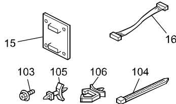
Optional Counter Interface Unit Type M12
