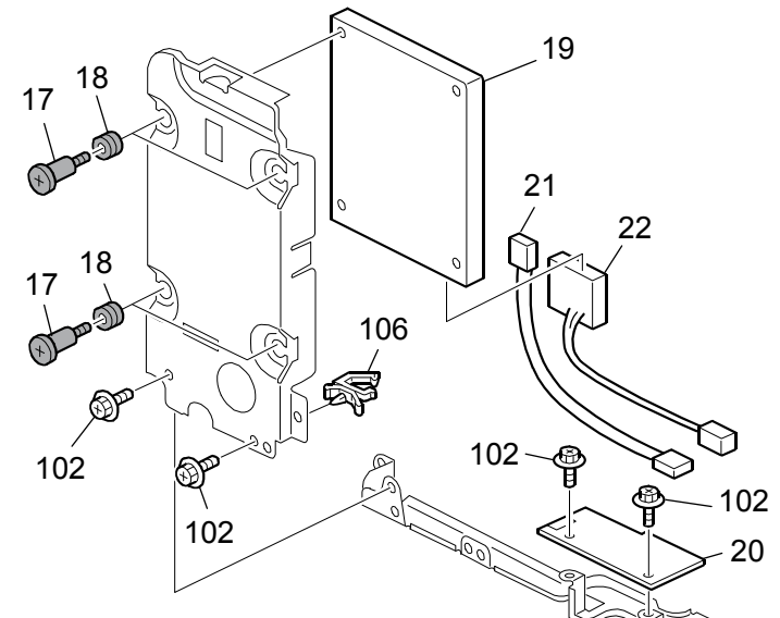
Gigabit Ethernet Board Type A (G874-01)
