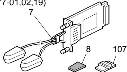
File Format Converter Type E (D377-04)
