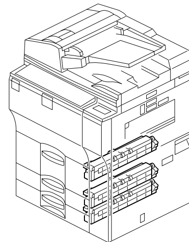
27. Paper Feed Unit 1 (D062/D063/D065/D066)
