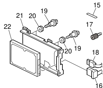
Hard Disk Drive Option Type P1
