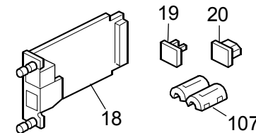
Card Reader Bracket Type 3352 (D593-61)
