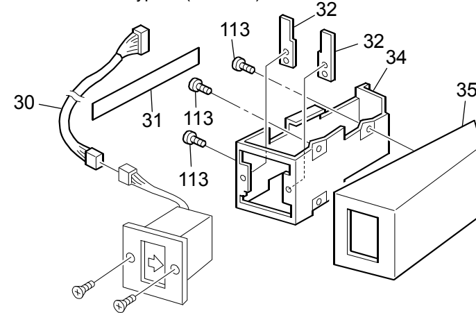
Key Counter Bracket Type H (A674-05)
