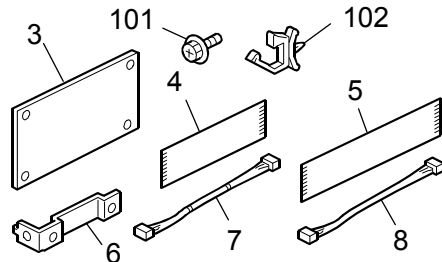
Optional Counter Interface Unit Type A (B870-11)
