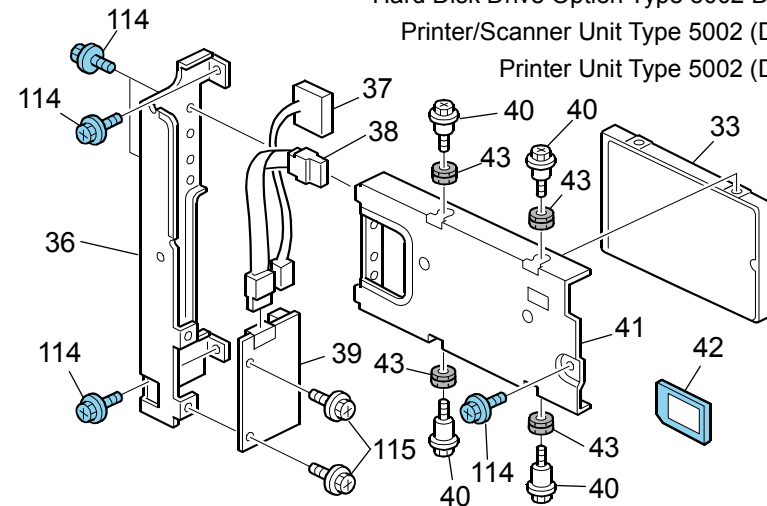
Hard Disk Drive Option Type 5002 D(640-11)
