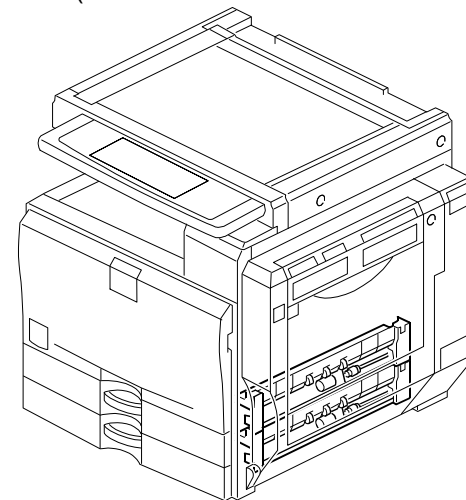
21. Paper Feed Section (D009/D011/D012/D013/D091/D092)
