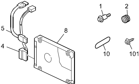
Hard Disk Drive Option Type M7 (D758-11)
