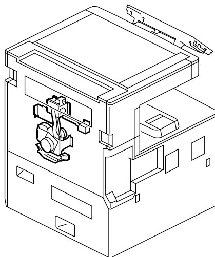
26. Drive Section 1 (D182/D183/D184)
