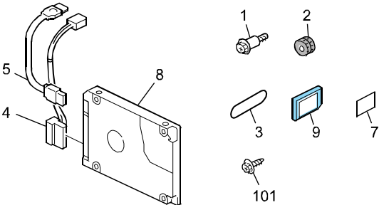
Printer Unit Type M7 (D757-32,33,34,35)
