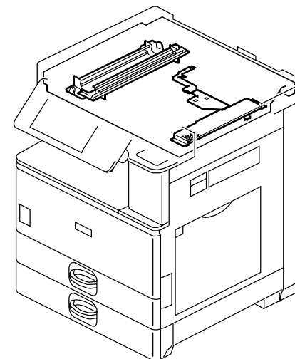
6. Scanner Section 2 (D182/D183/D184)
