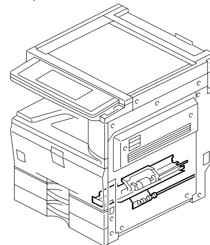
9. 1st Paper Feed Section (D017/D018/D019/D020/D084/D085)
