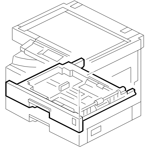
9. 1st PAPER TRAY (D010/D043)
