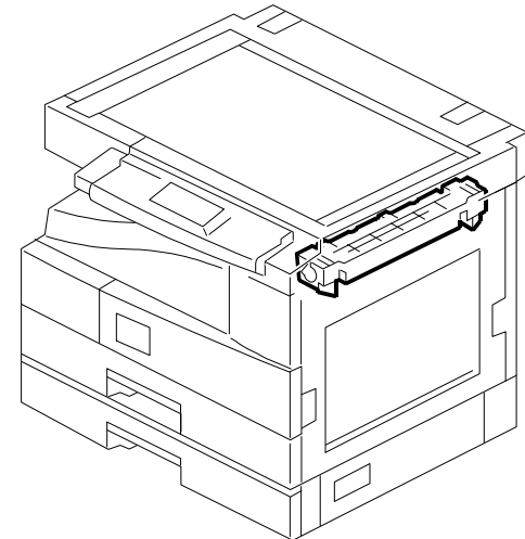
18. FUSING UNIT (D010/D043)
