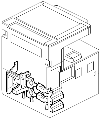
28. Drive Section 3 (D120/D121/D122/D139/D140/D141)
