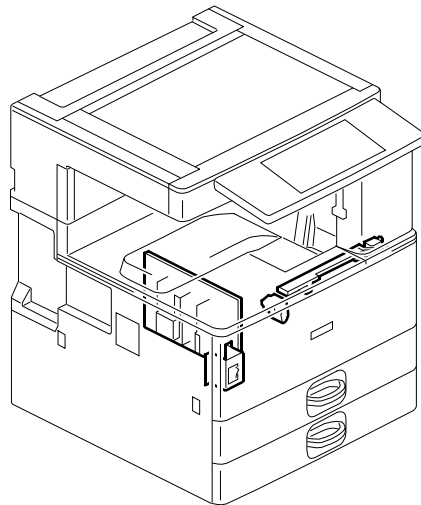
32. Electrical Section 4 (D120/D121/D122/D139/D140/D141)
