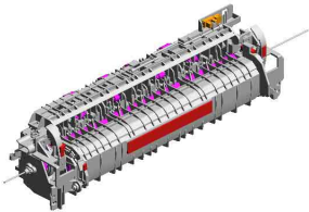
6.09543010N(x 2) SCREW:POLISHED ROUND/SPRING:M 3X10
