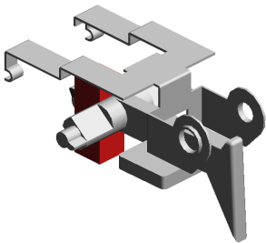
43.D1584043 STRIPPER PAWLS: SUB-ASS'Y
