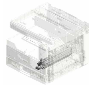
U008 PROCESSES AROUND PHOTOCONDUCTOR
