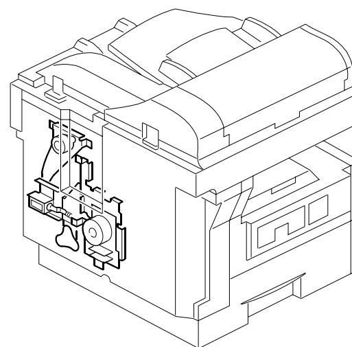
18. Drive Section (D115/D116)
