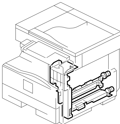
4. Paper Registration (D108)
