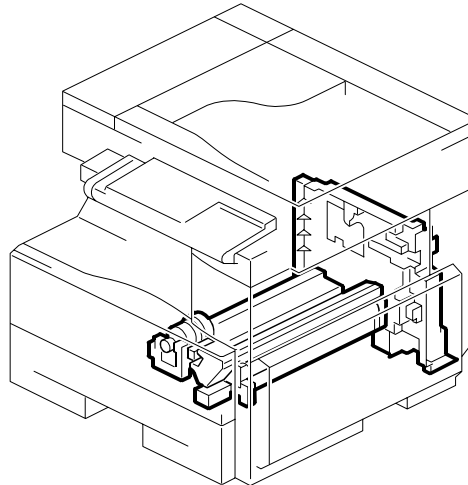
11. PCU Section (D108)
