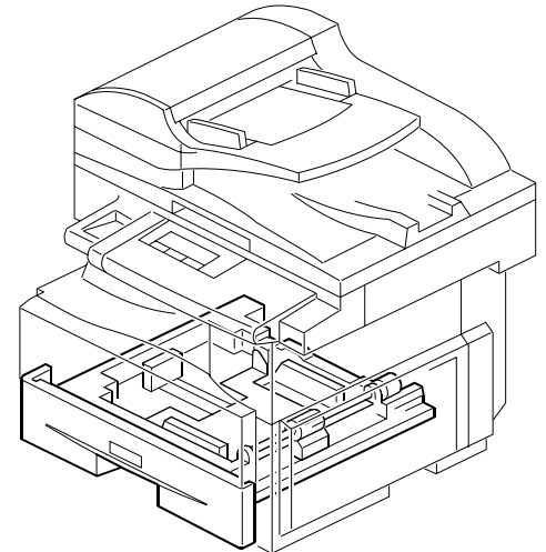
6. Paper Cassette (B284/B288)
