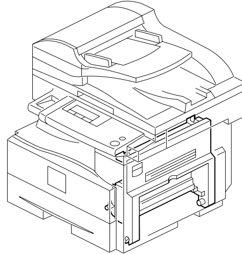
5. Transport Section (B284/B288)
