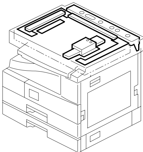
4. Optics Section 1 (B24562)
