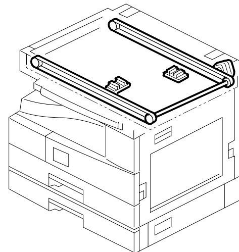
6. Optics Section 3 (B24562)
