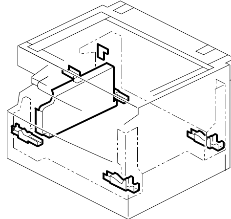
23. Frame Section 1 (B282-62/B283-62)
