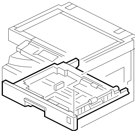
8. Paper Cassette (B282-62/B283-62)
