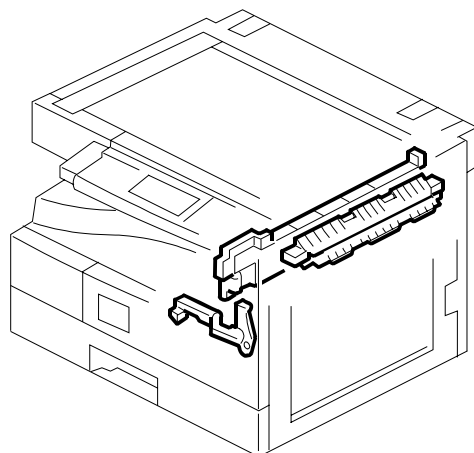
16. Paper Exit Section (B282-62/B283-62)
