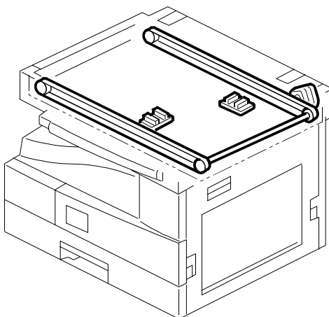
5. Optics Section 3 (B282/B283)
