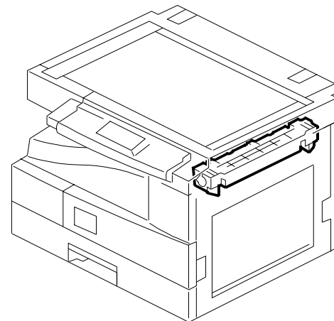
15. Fusing Unit (B282/B283)
