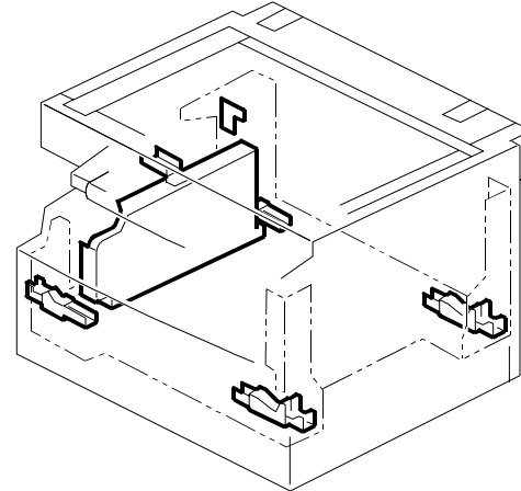
23. Frame Section 1 (B282/B283)
