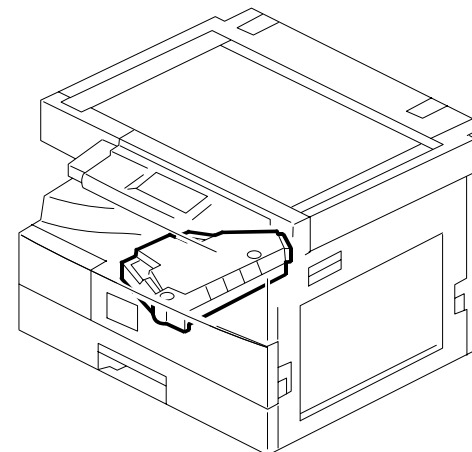
6. LASER UNIT (B28264/B28364)
