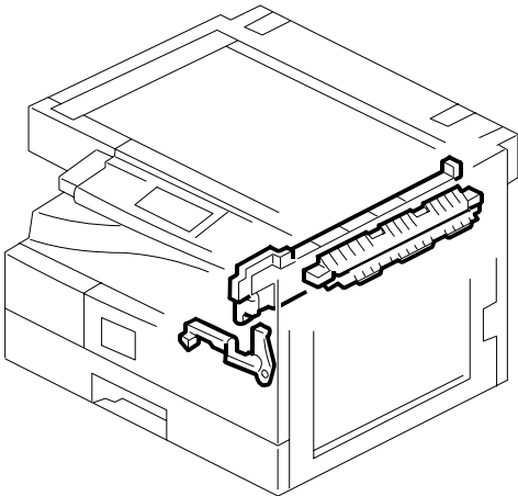
16. PAPER EXIT SECTION
