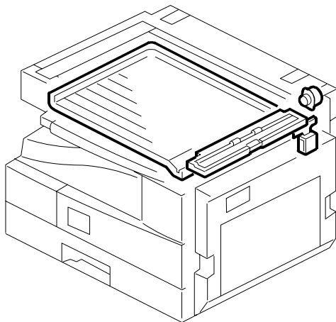
19. DUPLEX UNIT 3 (B28264/B28364)
