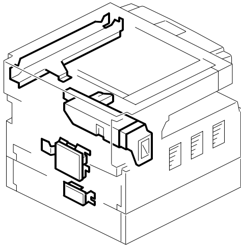
20. Electrical Section 2 (B24561)
