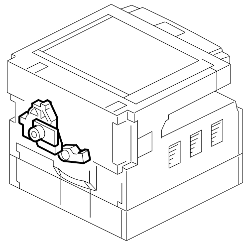
18. Drive Section (B24561)
