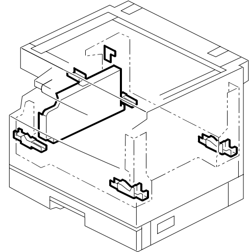
21. Frame Section 1 (B24561)
