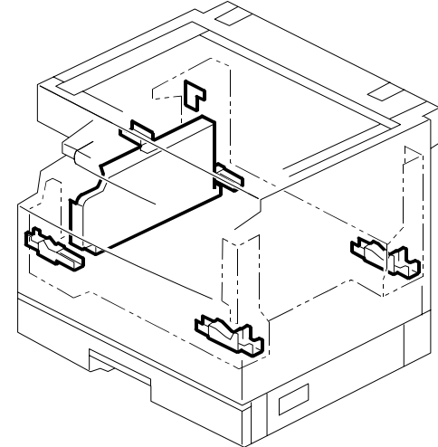
21. FRAME SECTION 1 (B24521)
