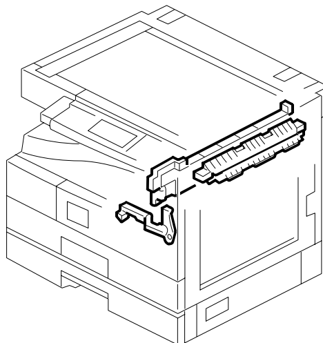
17. PAPER EXIT SECTION (B24521)
