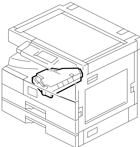
7. LASER UNIT (B24521)
