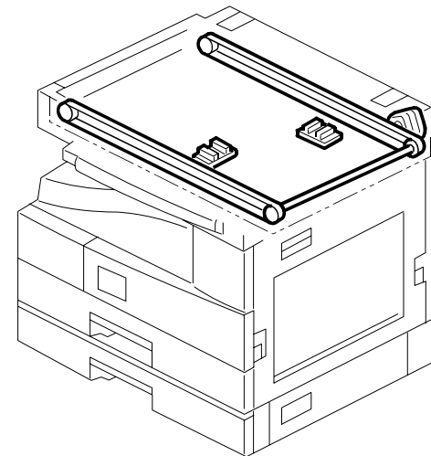
6. OPTICS SECTION 3 (B24521)
