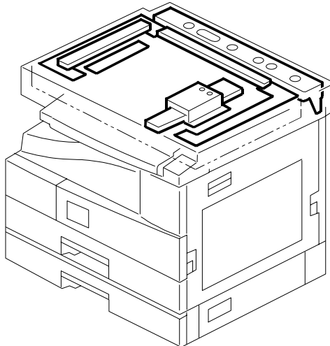
4. OPTICS SECTION 1
