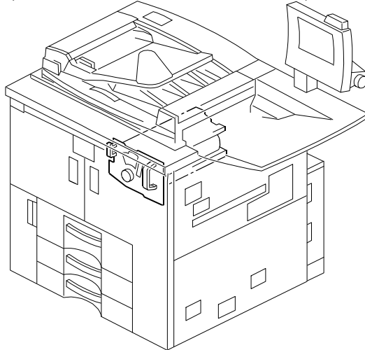
40. PCU 1 (B234/B235/B236/D101/D102/D103)
