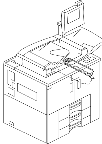
35. Toner Hopper Section (B234/B235/B236/D101/D102/D103)
