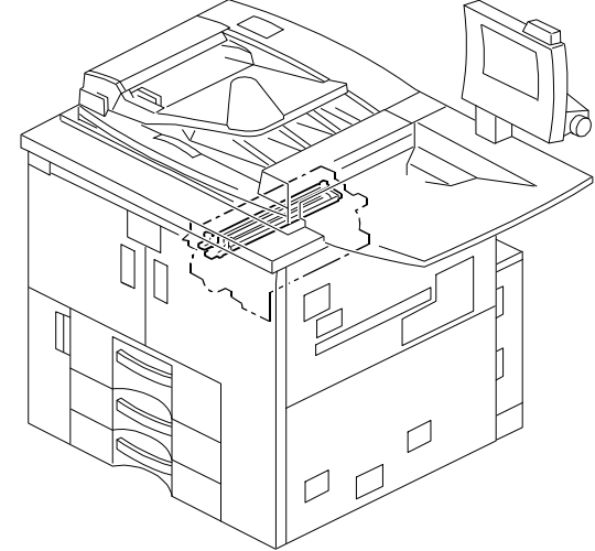
36. Charge Corona Unit 1 (B234/B235/B236/D101/D102/D103)
