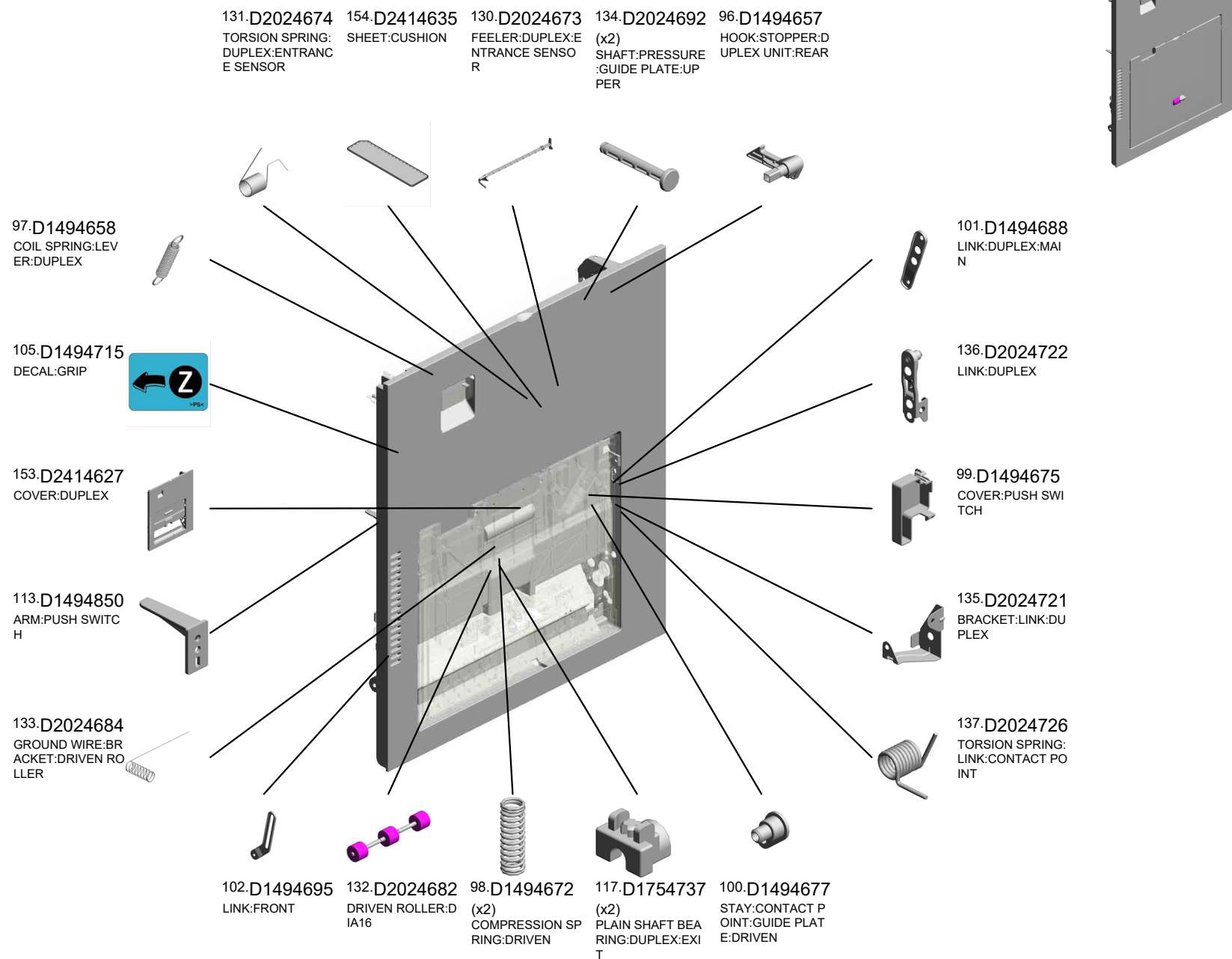
53.D0BK4553 DUPLEX UNIT:IMC 2000-2500
