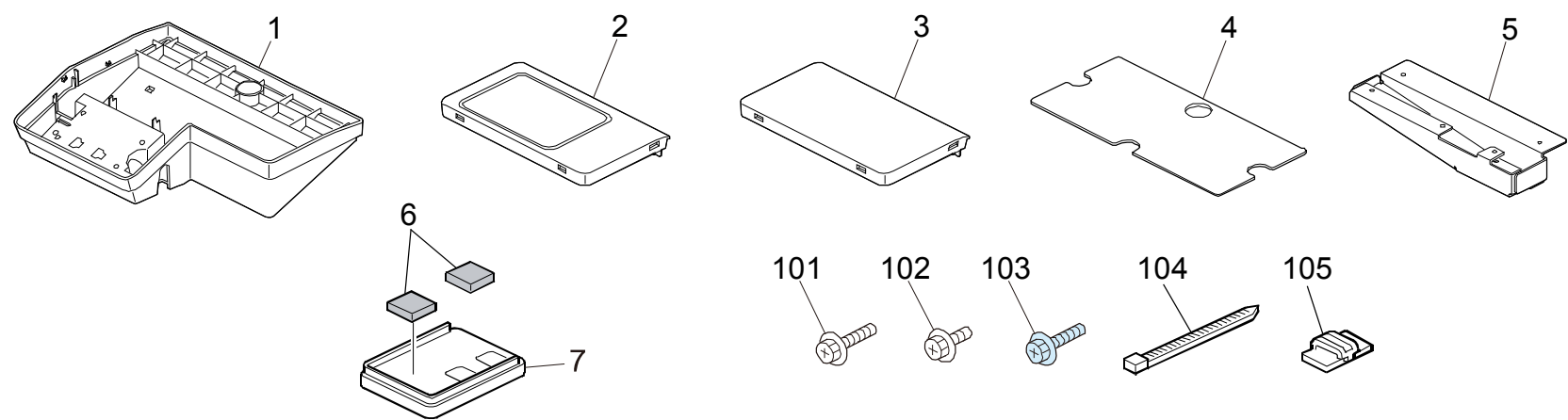
NFC Card Reader Type M37 (D3GF34)
