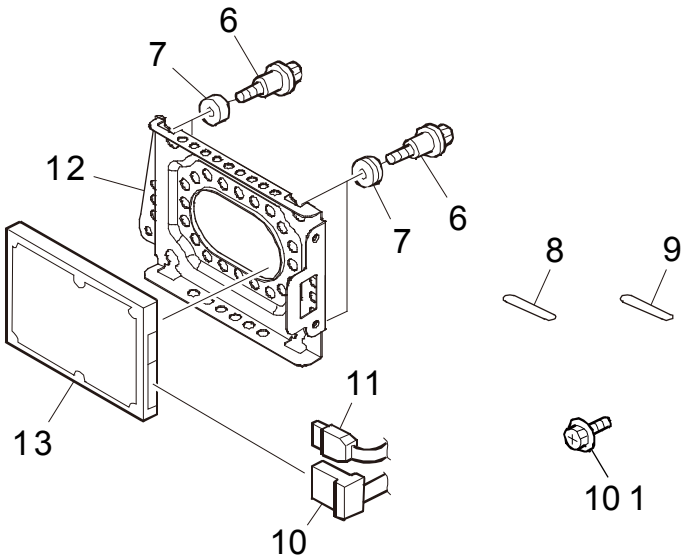
Enhanced Security HDD Option Type M12 (D3A602)
