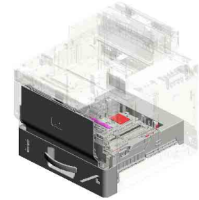
U004 PAPER FEED
