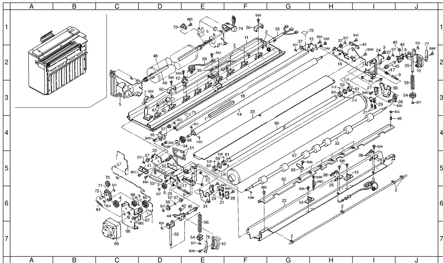
FIG. 16 LOWER FIXING SECTION
