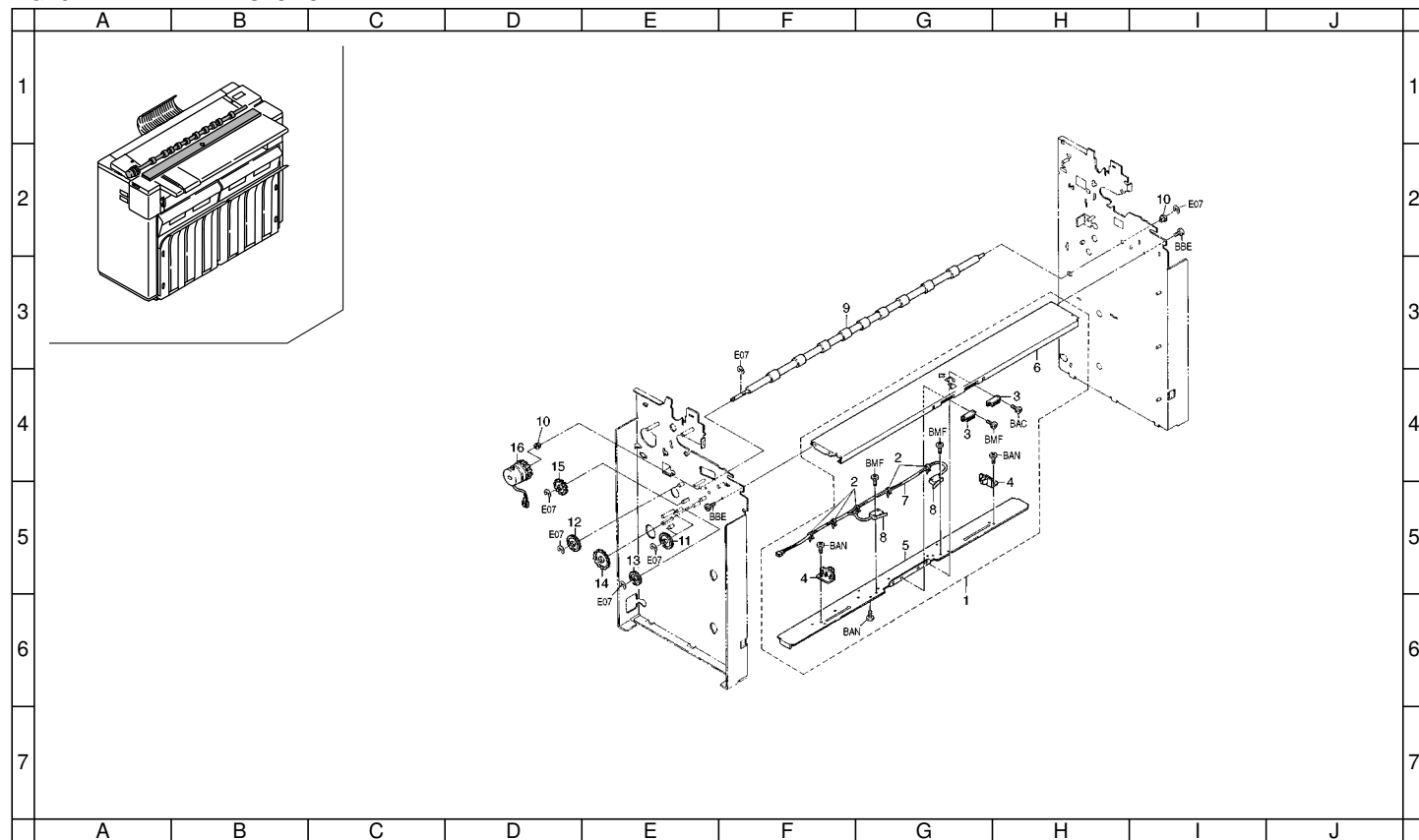
FIG. 3 PAPER FEED-IN SECTION 1
