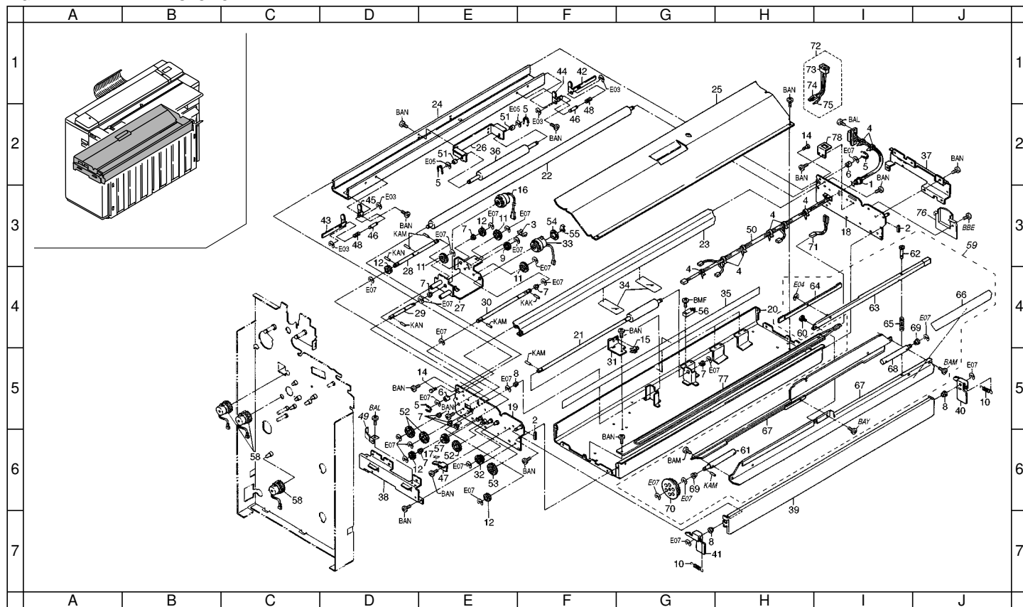
FIG. 4 PAPER FEED-IN SECTION 2
