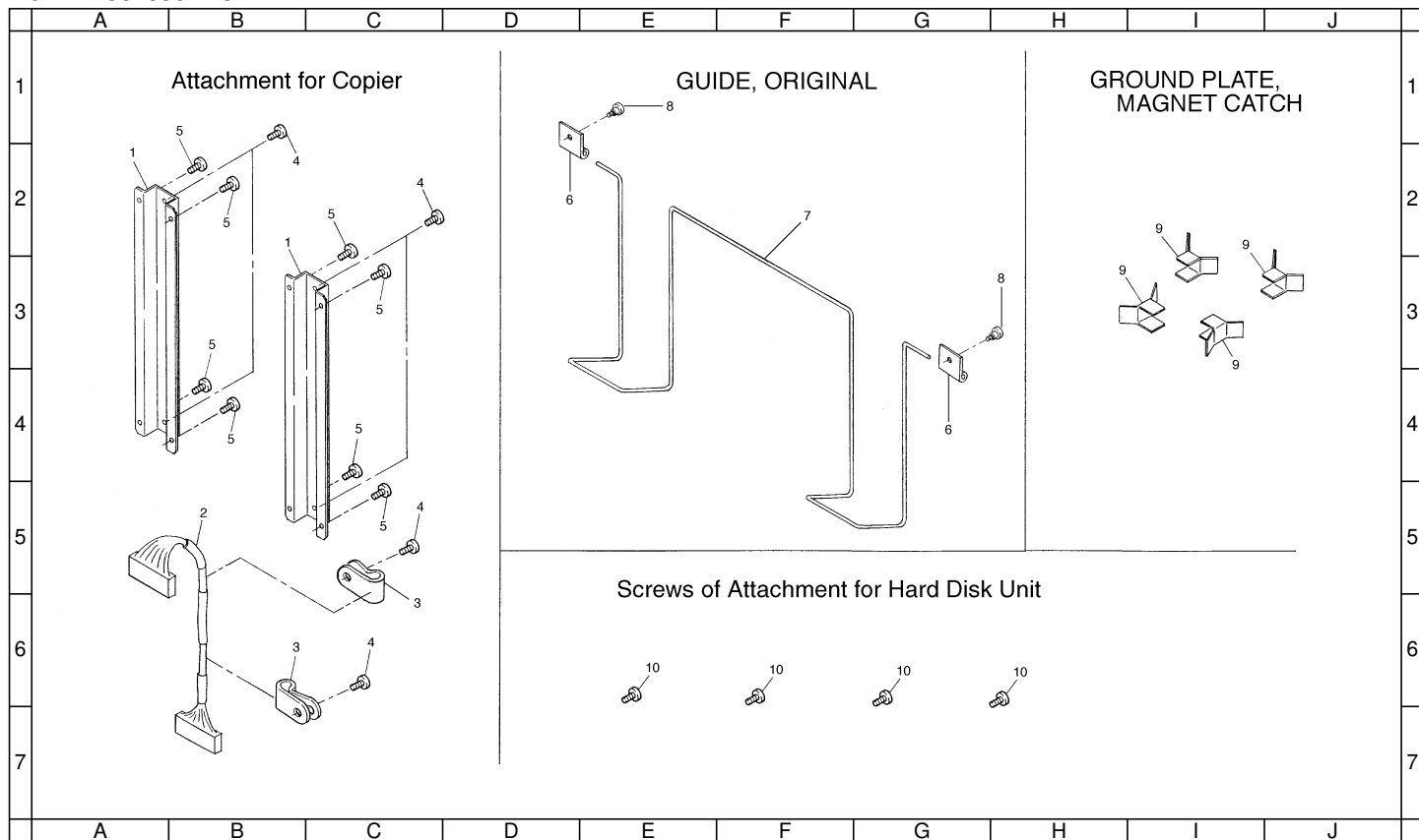
FIG. 2 ACCESSORIES
