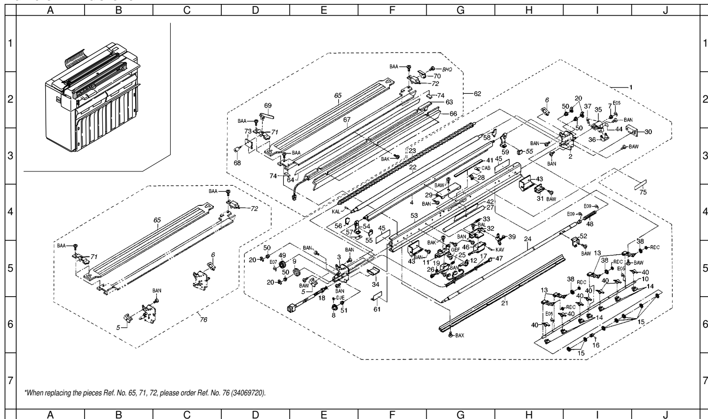
FIG. 13 CLEANING SECTION 1
