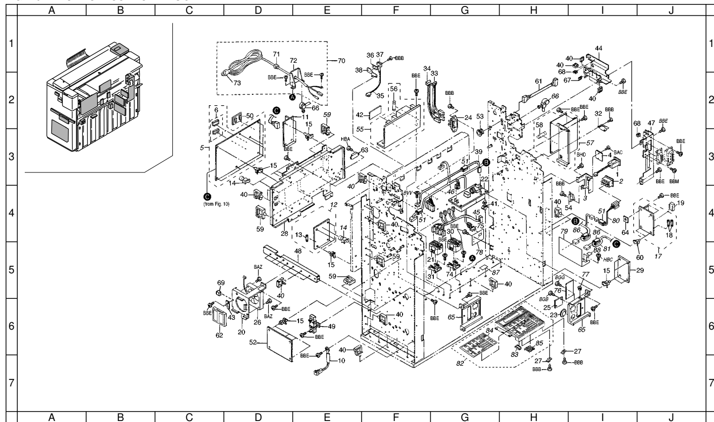
FIG. 20 ELECTRICAL COMPONENTS 3
