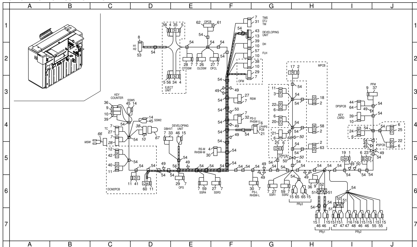
FIG. 18 ELECTRICAL COMPONENTS 1
