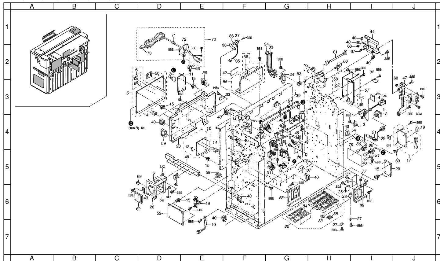
FIG. 20 ELECTRICAL COMPONENTS 3
