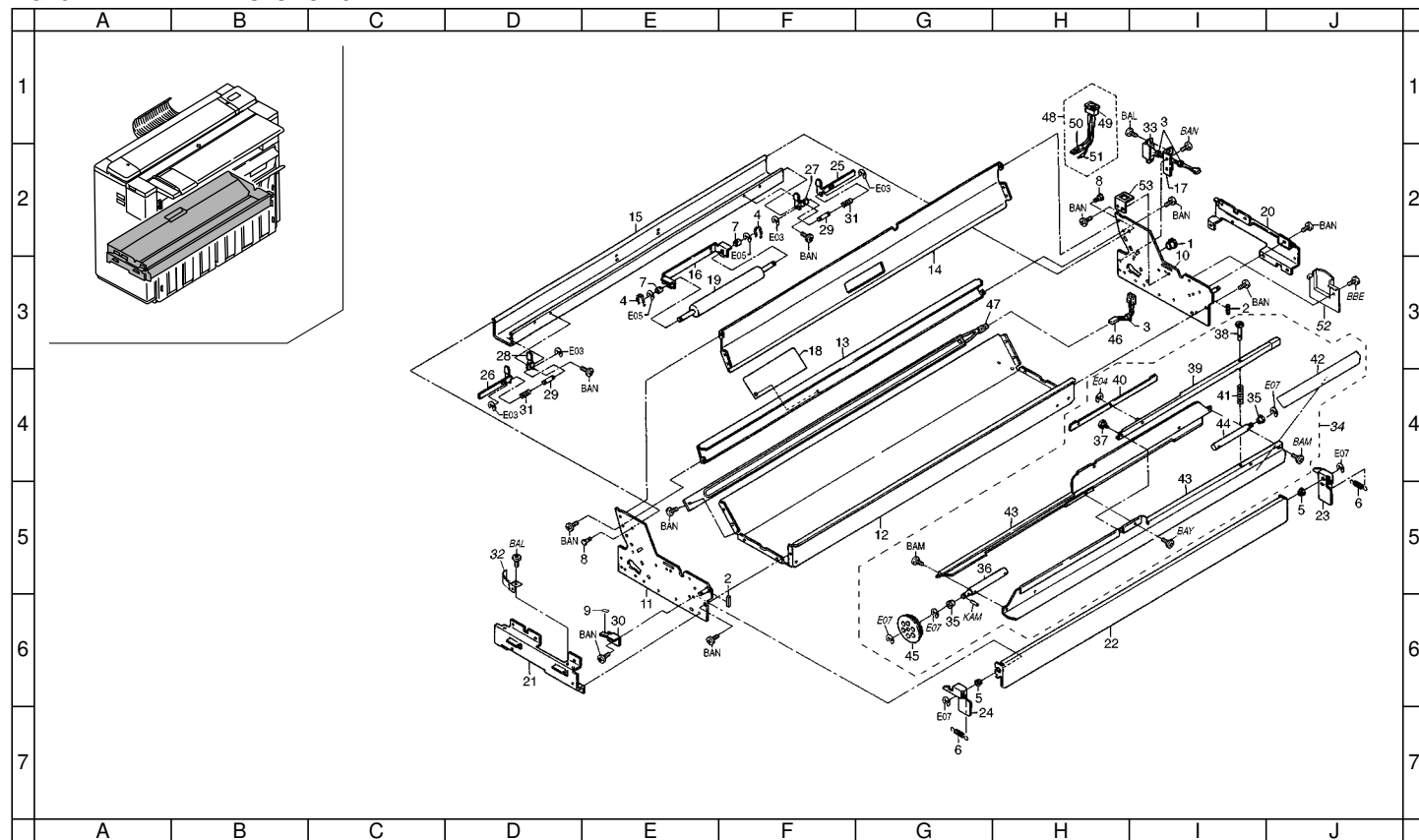
FIG. 5 PAPER FEED-IN SECTION 3
