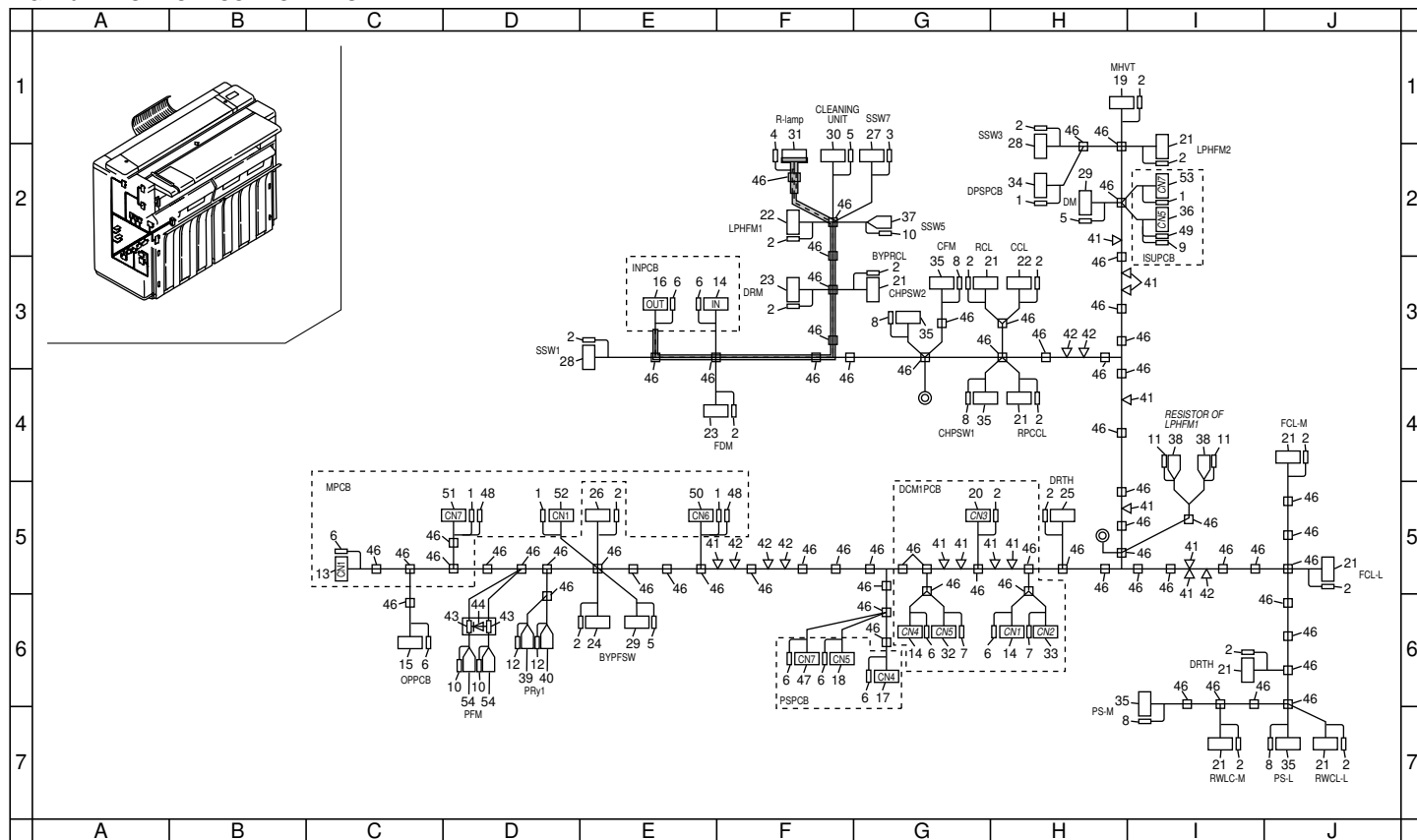
FIG. 19 ELECTRICAL COMPONENTS 2
