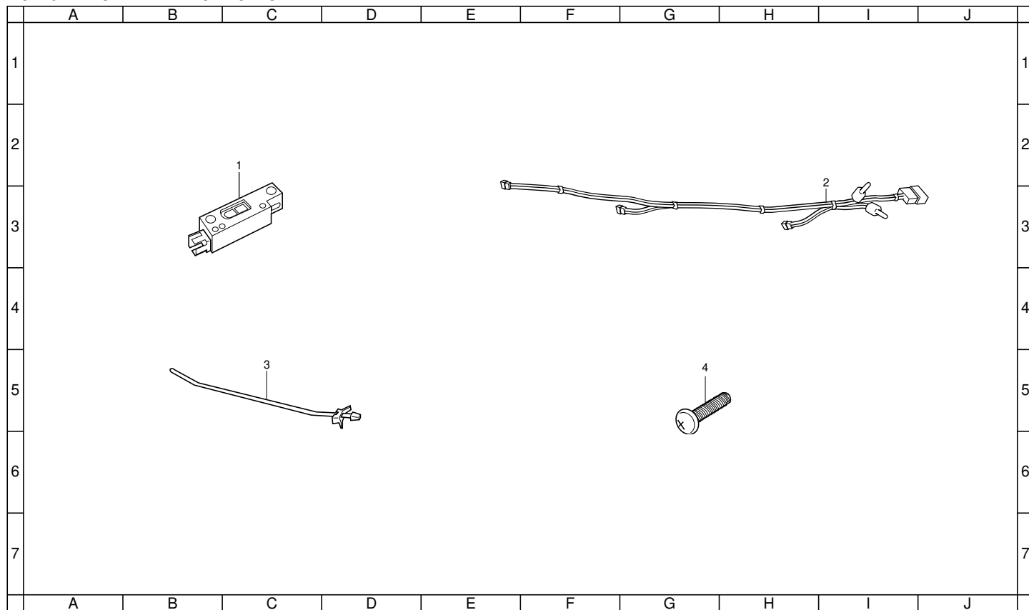
FIG. 25 ATTACHMENT KIT FOR ROLL UNIT
