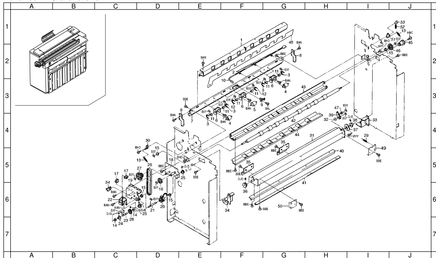
FIG. 6 CUTTER, EJECT SECTION
