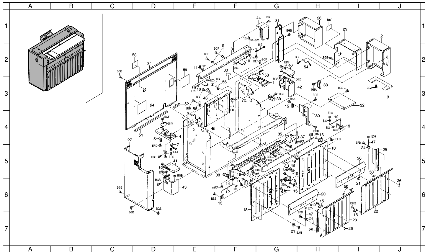
FIG. 1 EXTERIOR COVERS
