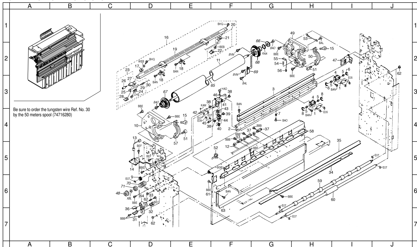
FIG. 7 IMAGE FORMATION SECTION 1
