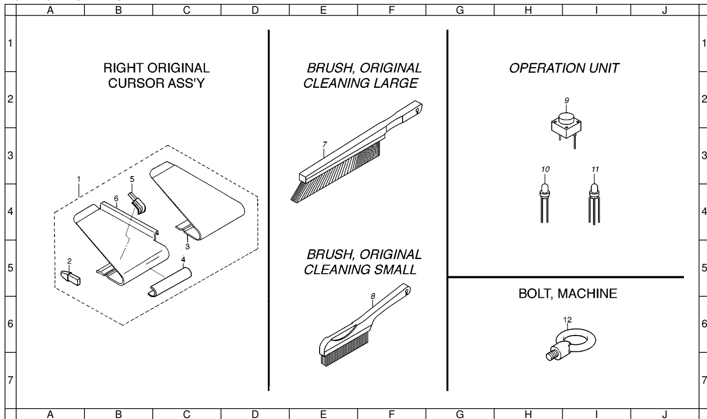
FIG. 24 SERVICE PARTS
