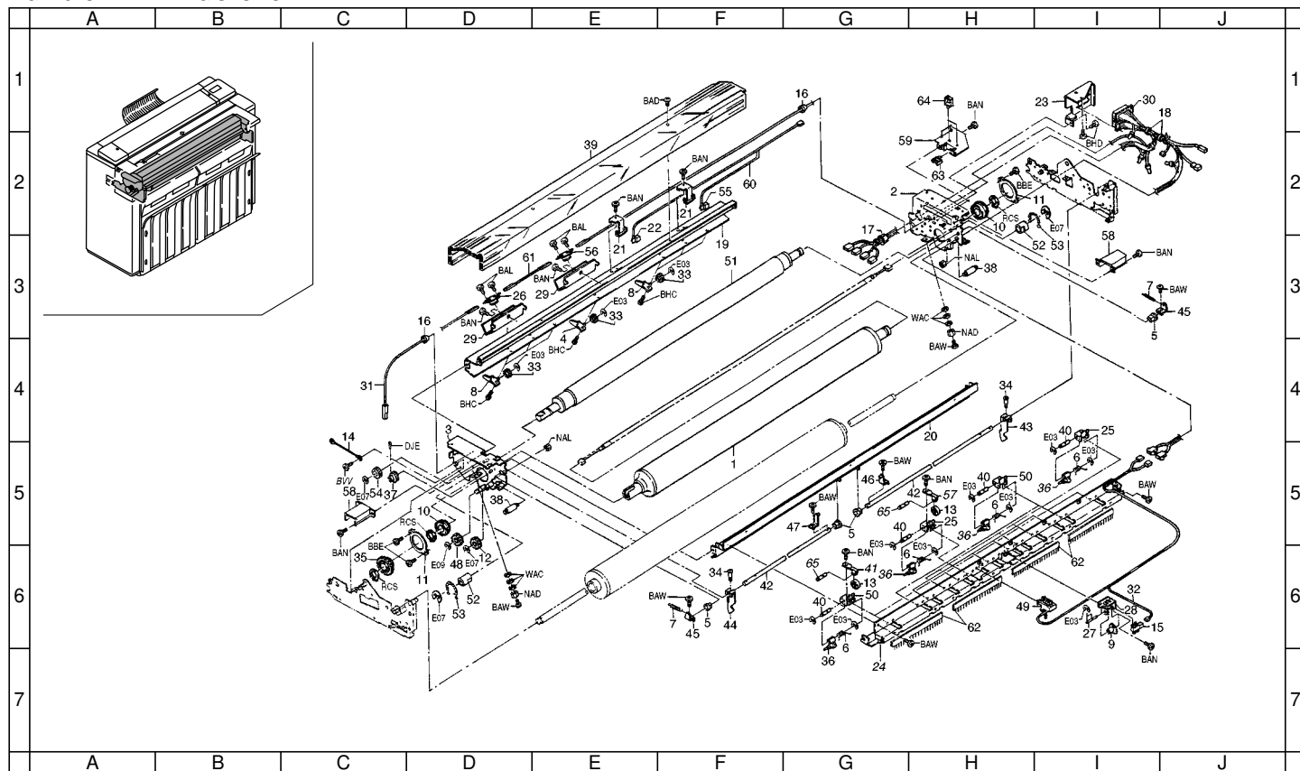
FIG. 15 UPPER FIXING SECTION
