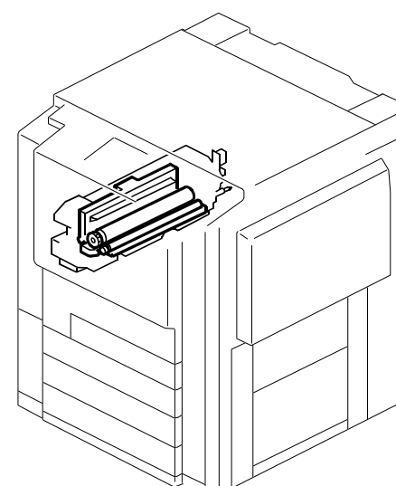
36.FUSING UNIT 3 (A257/A269)
