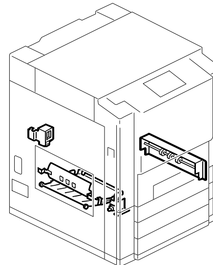
39.PAPER INVERTOR SECTION (A257/A269)
