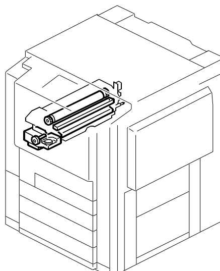
35.FUSING UNIT 2 (A257/A269)
