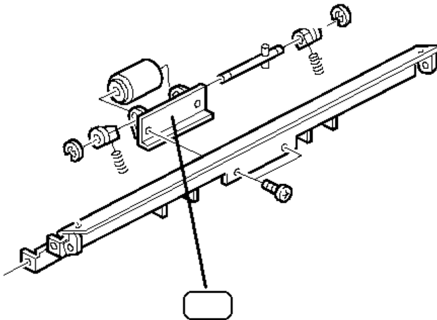
Separation Roller Spacer
