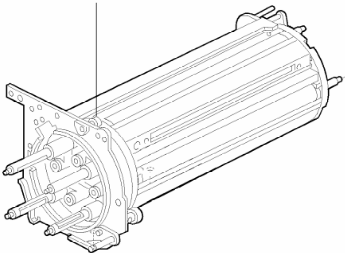
Roller Development Unit Plate
