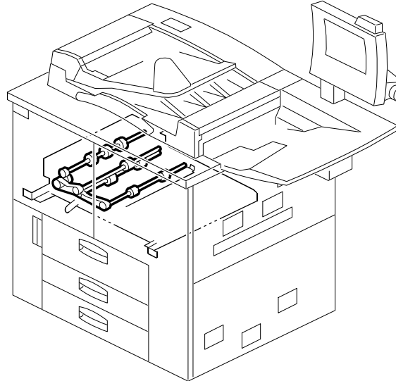
56.DUPLEX UNIT 5 (A294)
