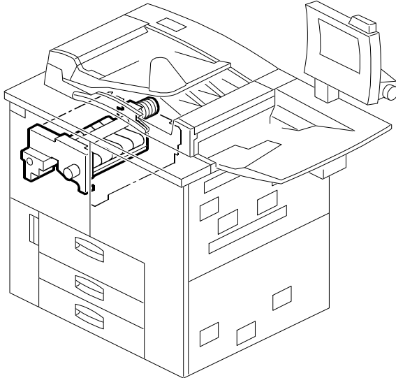
49.PAPER EXIT SECTION 2 (A294)
