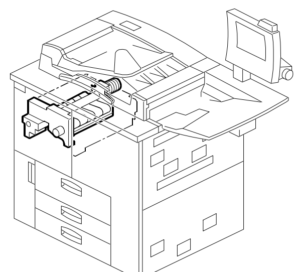
48. PAPER EXIT SECTION 1 (A294)
