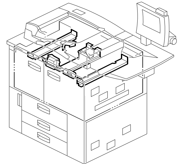
69.FRAME SECTION 2 (A294)
