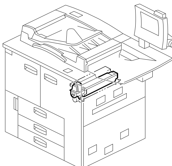
35.TONER HOPPER SECTION (A294)
