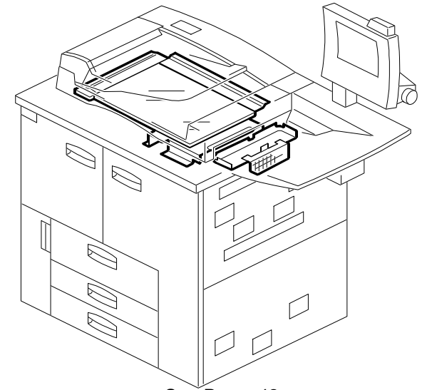
15.OPTICS SECTION 1 (A294)
