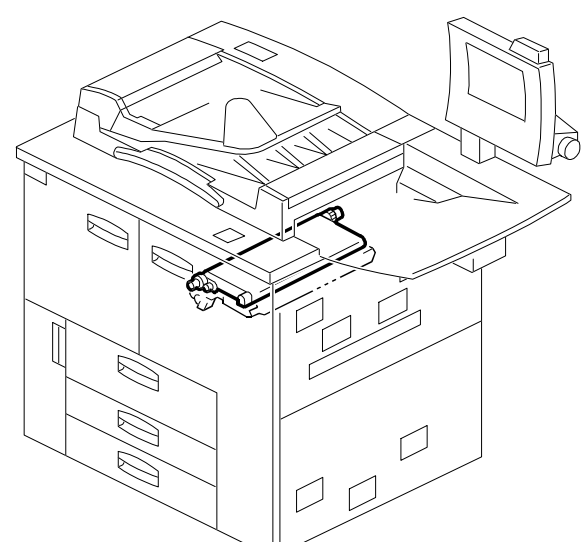
42.TRANSFER BELT UNIT 1 (A294)
