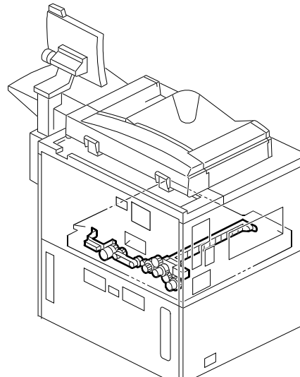
53.DUPLEX UNIT 2 (A294)
