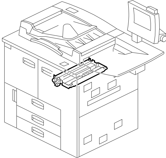
43. TRANSFER BELT UNIT 2 (A294)
