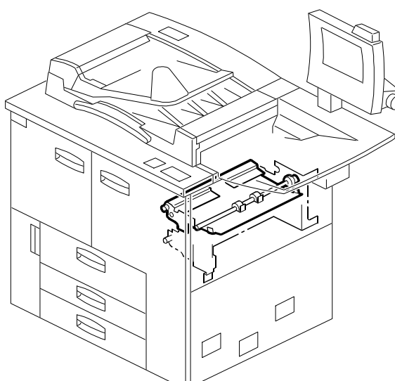
29.PAPER REGISTRATION 2 (A294)
