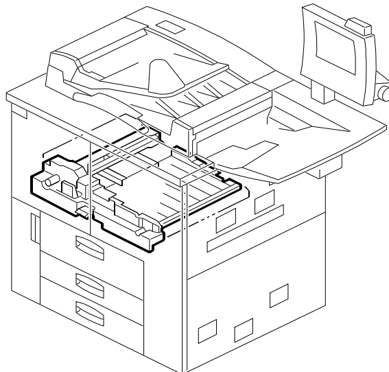
52.DUPLEX UNIT 1 (A294)
