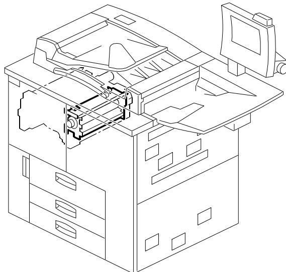
46. FUSING UNIT 3 (A294)
