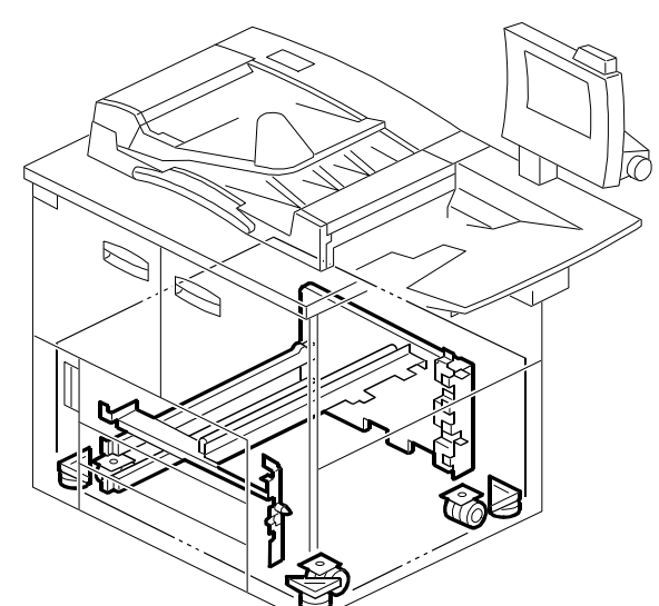
72.FRAME SECTION 5 (A294)
