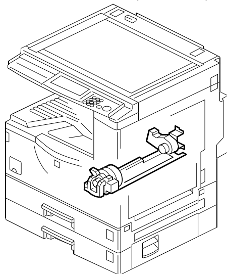
13.TONER HOPPER UNIT (A265/A267)
