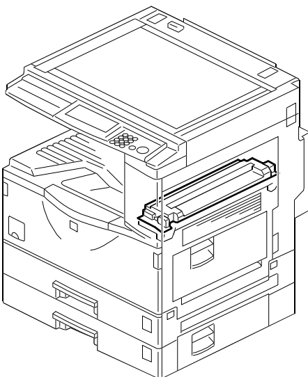
17.FUSING UNIT 1 (A265/A267)
