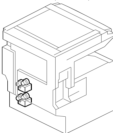
22.DRIVE SECTION 3 (A265/A267)
