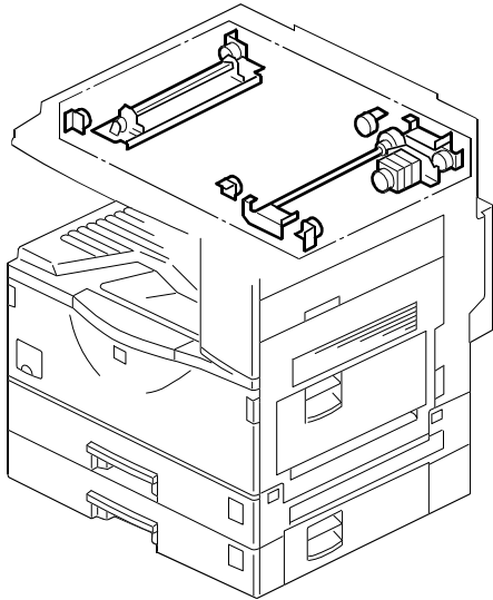
7.OPTICS SECTION 3 (A265/A267)
