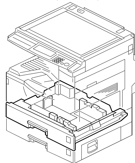
15.PAPER TRAY 1 (A265/A267)
