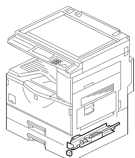
12.PAPER FEED SECTION 3 (A265/A267)
