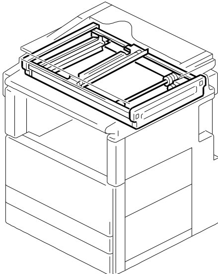
10. Optics Section 2 (A193)
